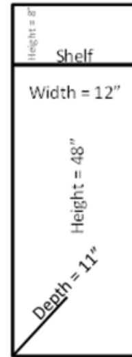
Locker Dimensions
